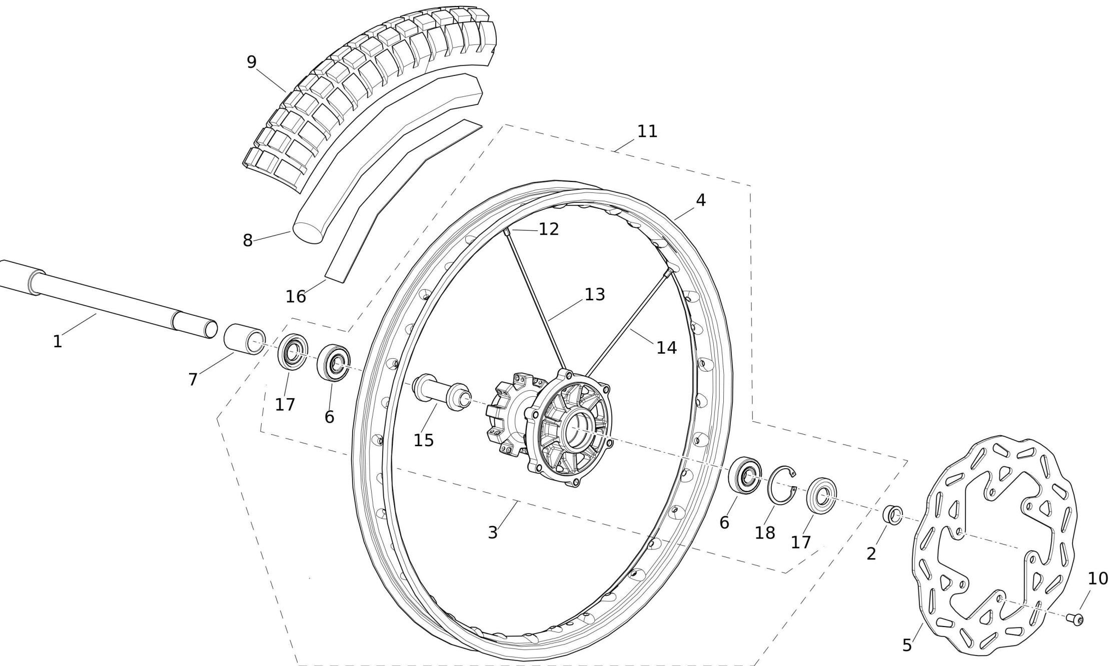
Front wheel
