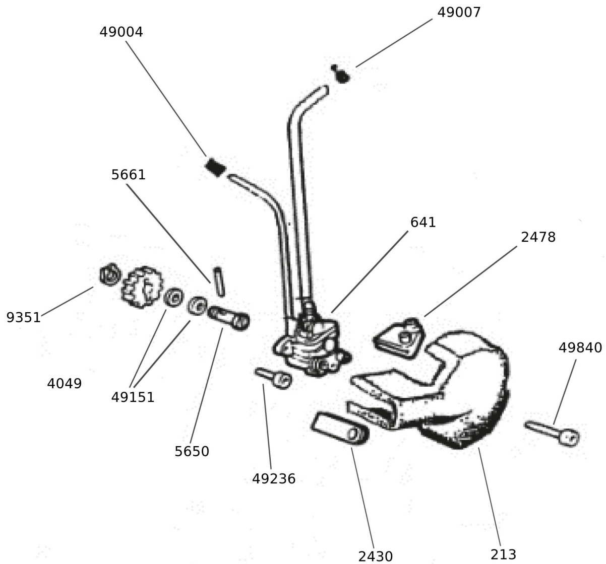
Oil pump
