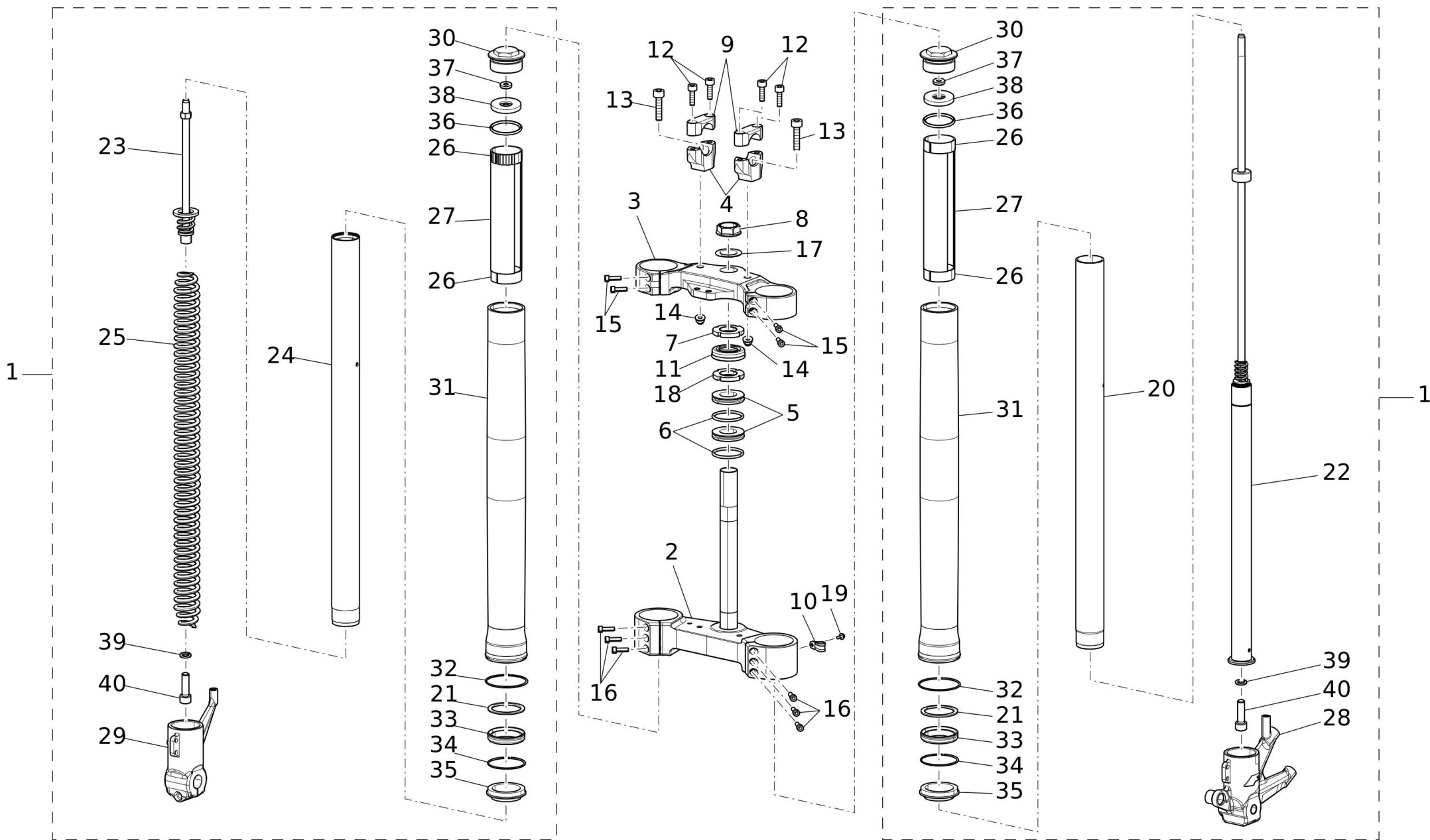
3 - Fork Scrambler (CABALLERO 500 E5 MY21-MY22)
