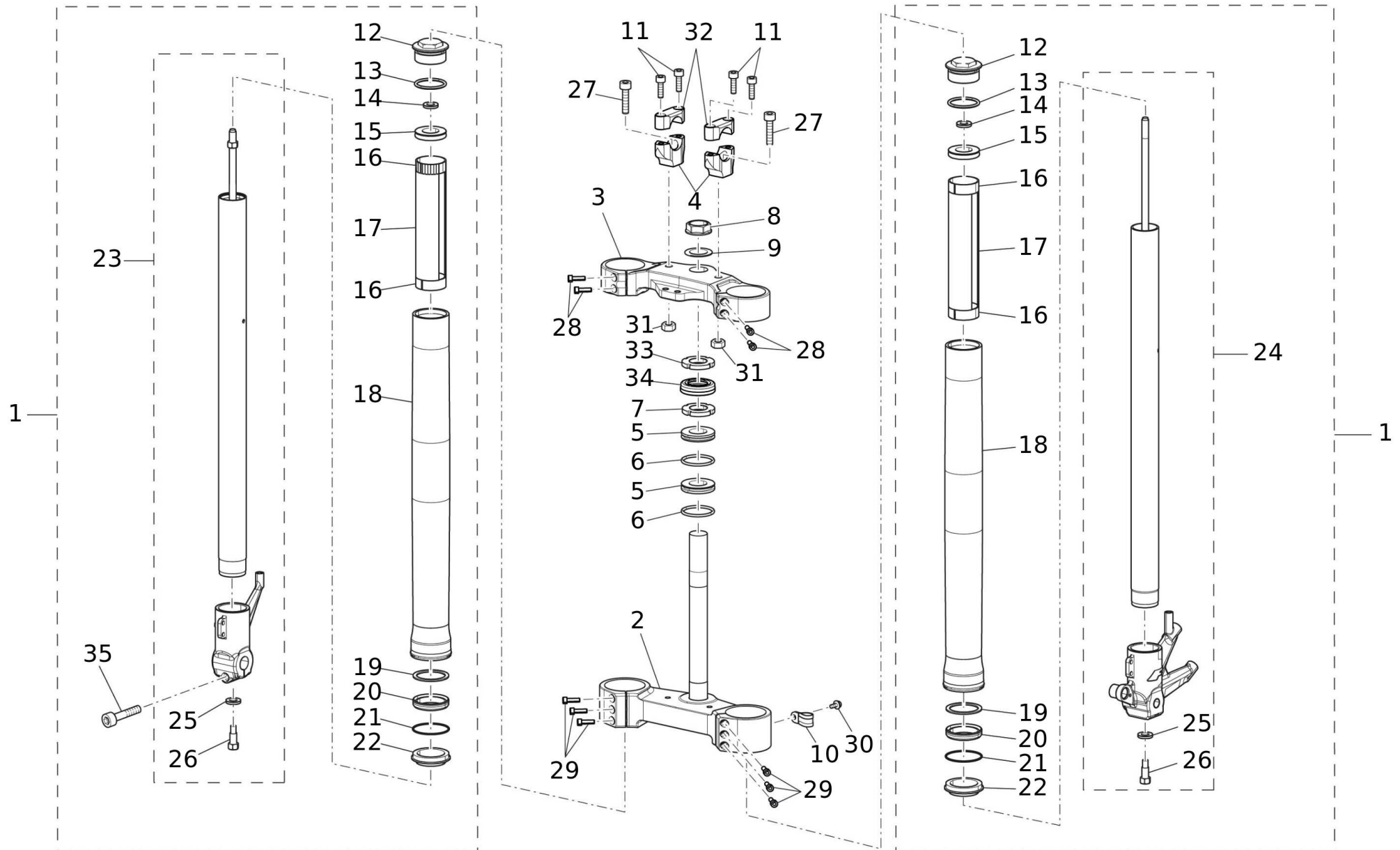
3 - Front fork Scrambler (CABALLERO 125 MY2021-22)
